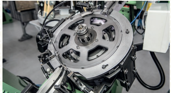
RP8LD with roller block slide in combination with special bushing loader. Bushing loading and rolling up to diameter 16 mm.
